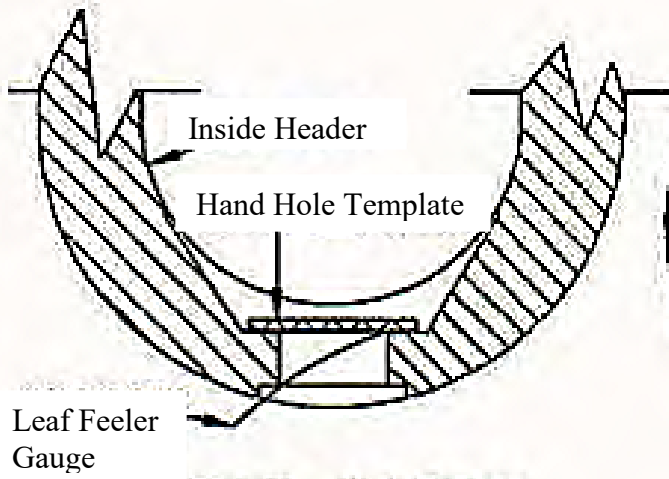
SEAT TAPER
